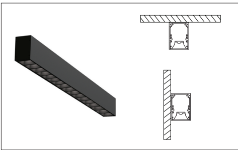
SURFACE MOUNT, WALL FLUSH
